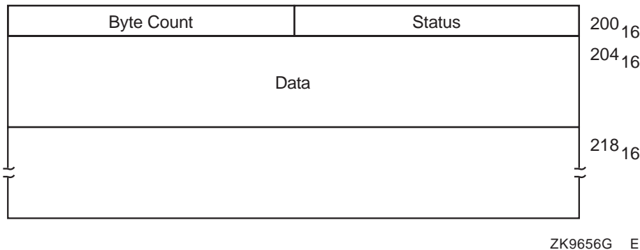
Figure 6-1 Buffer Layout
